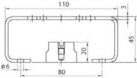
Bracket for Rotex Actuator models ECV50 through ECV175
