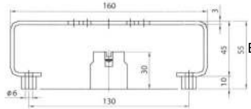
Bracket for Rotex Actuator models ECV200 through ECV350
